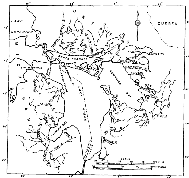
Fig. 2. The Lake Huron watershed showing major tributaries.
